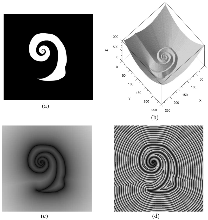
Fig. 2. The image of a spiraled shape (a) and representations of the distance transform of its border, where the height of the surface in (b) or the brightness in (c) are proportional to the smallest distance of each point to the border pixels. In (d) there is a visualization of iso-distance curves.
