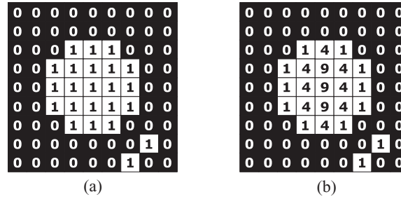
Fig. 6. Example of the 1D transformation common to independent scanning EDTs. (a) The input image F ; (b) its 1D EDT G along each row.
