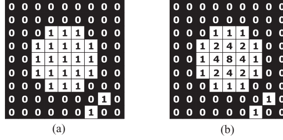
Fig. 1. Numerical example of distance transform. In (b) there is the Euclidean distance of each pixel to the nearest black pixel. The distance values are squared so that only integer values are stored.
