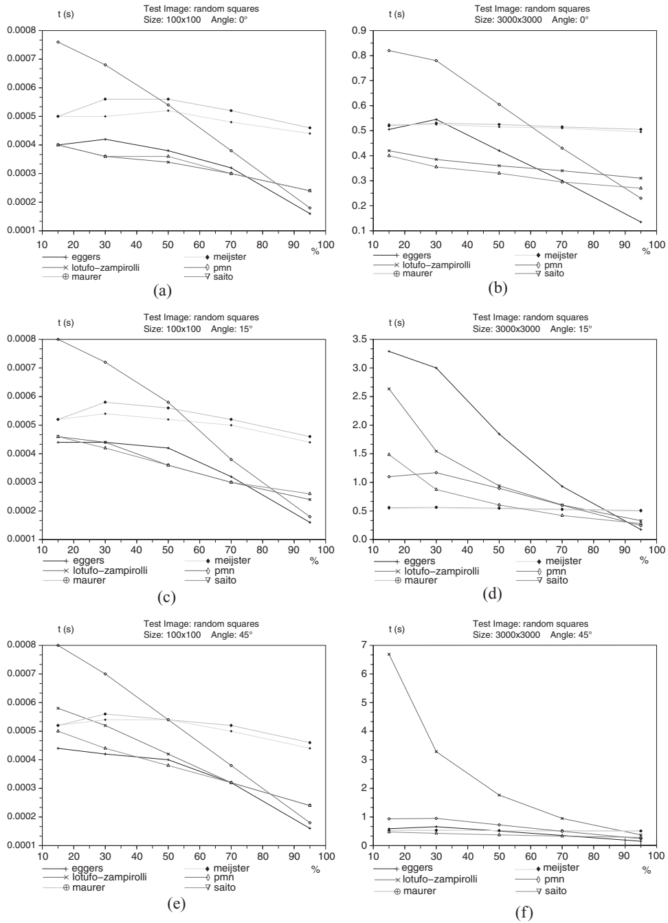
Fig. 28. Performance of EDT methods for random squares, varying percentage of black pixels (abscissas) and fixing orientation at 0^\circ in (a) and (b), 15^\circ in (c) and (d), and 45^\circ in (e) and (f), for 100 \times 100 images (left column) and 3000 \times 3000 (right column).
