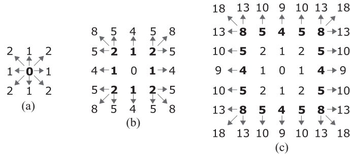
Fig. 16. First three iterations of Eggers' sufficient propagation d_\infty . Bold values indicate pixels in the contour set. Main contour pixels are those propagating to three pixels, and the minor are those propagating only to a single one. An indirect pixel N_k(p) of a main pixel p having directional index k will be a main pixel during the next iteration. The remaining ones will be minor pixels.
