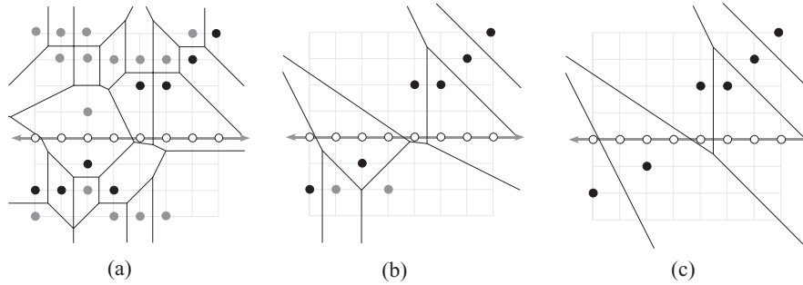
Fig. 10. In (a) there is the VD of all sites represented by solid dots. Sites marked in gray are not relevant for computing the EDT within the gray line, since their VR do not intercept this line. The sites marked in (a) are discarded to generate (b), keeping only the closest sites along each column. In (b) the marked sites are removed, which do not pass a certain test of bisector intersection. In (c), there is the VD of the relevant sites. The intersection of the complete VD (a) with the line is not altered in the partial VDs (b) and (c).
