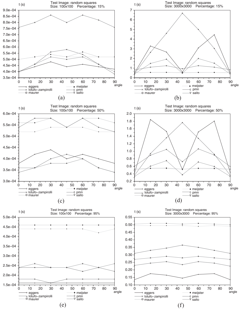
Fig. 29. Performance of EDT methods for images of random squares, varying the angle (abscissas), and fixing the percentage of black pixels at 15% in (a) and (b), 50% in (c) and (d), and 95% in (e) and (f), for 100 \times 100 images (left column) and 3000 \times 3000 (right column).
