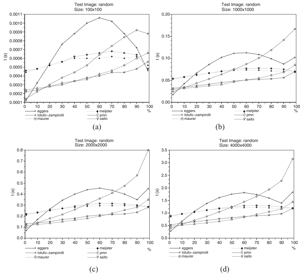
Fig. 25. Performance of EDT methods for images with varying percentage of white pixels at random locations. Plots are shown for sizes 100 \times 100 (a), 1000 \times 1000 (b), 2000 \times 2000 (c), and 4000 \times 4000 (d).
