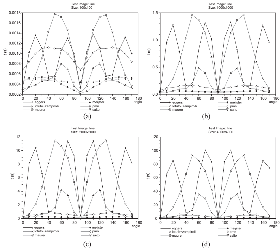
Fig. 26. Performance of EDT algorithms for images with a single line in different angles. Plots are shown for sizes 100 \times 100 (a), 1000 \times 1000 (b), 2000 \times 2000 (c), and 4000 \times 4000 (d).
