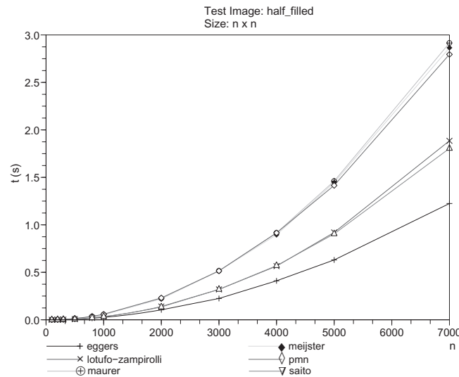
Fig. 24. Performance for the half-filled image.
