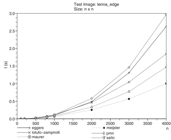
Fig. 23. Performance for Lenna's contours.
