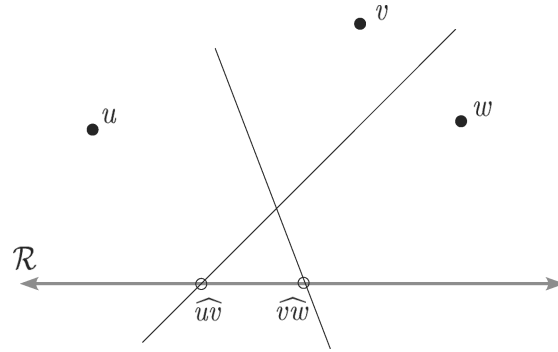
Fig. 11. The Voronoi region of v does not intercept line \mathcal{R} if \widehat{uw}_x \geq \widehat{vw}_x .
