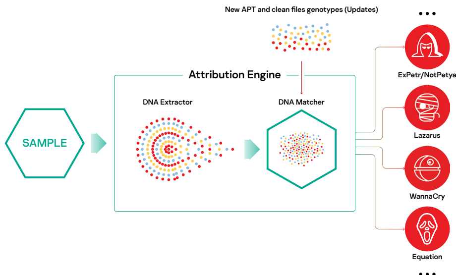
Picture 4. Kaspersky Threat Attribution Engine
