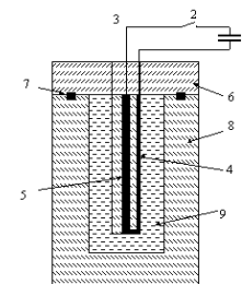
Experimental detection of "strange" radiation and transformation of chemical elements (2002)
