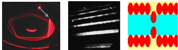
Laser whiskers in soap films (2002)
