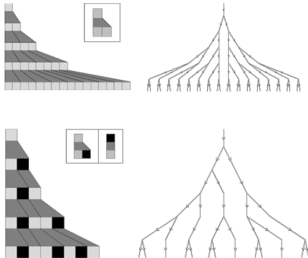
Figure 7: A pair of nontrivial string substitution systems exhibiting causal invariance ( A \rightarrow AA and \{A \rightarrow AB, B \rightarrow A\} , respectively), since in both cases the combinatorial structure of the causal graph is independent of the order in which the string substitutions get applied. Adapted from S. Wolfram, A New Kind of Science , page 500.
