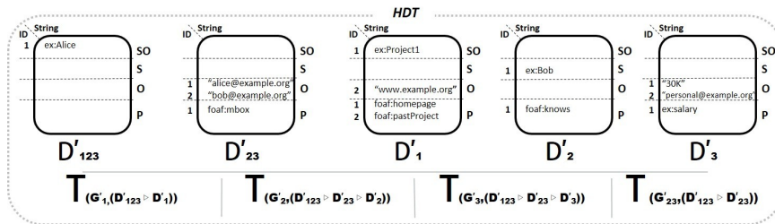
Figure 8.11: HDT_{crypt-D} , extracting non-overlapping dictionaries and triples.
