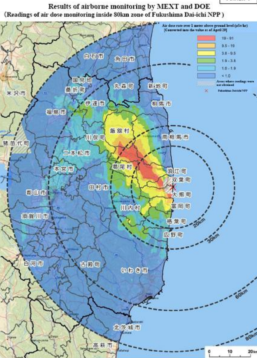
Figure 6B: MEXT and DoE map of dose rates from airborne measurements collected between April 6 and April 29, 2011
