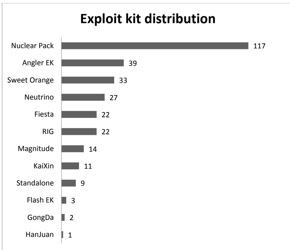
Graph I - Distribution of exploit kits
