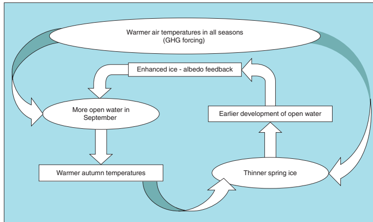
Figure 3: A complex set of interconnected processes lead to the Arctic's rapidly shrinking sea ice cover, according to Mark Serreze [NSIDC, CIRES]. Image adapted from Stroeve et al. , 2011.
