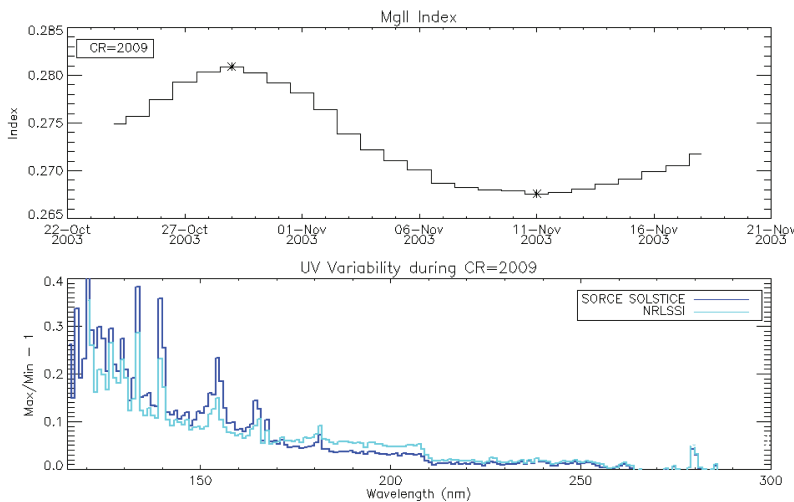
Figure 5: The solar spectral variability is shown for one 27-day solar rotation. Marty Snow [LASP].
