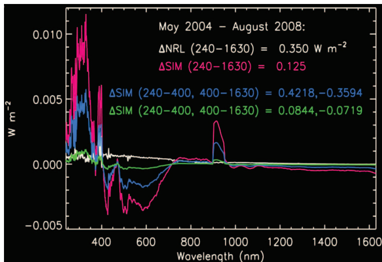
Figure 2: Several speakers addressed differences between the SIM spectral irradiances and UV measurements or solar models. Judith Lean discussed the expected impacts of the SIM-reported irradiances—if correct—on climate and atmospheric temperatures, and showed large differences between the SIM data and the NRL solar model from times of an active to quiet Sun.
