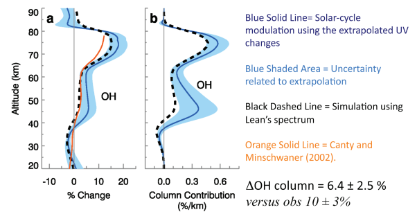
Figure 8: Model simulations using different spectral irradiance scenarios. The solar cycle change in the OH abundance measured by the Aura's Microwave Limb Sounder (MLS) instrument is in agreement with simulations using SORCE/SIM SSI variability per King-Fai Li [JPL].
