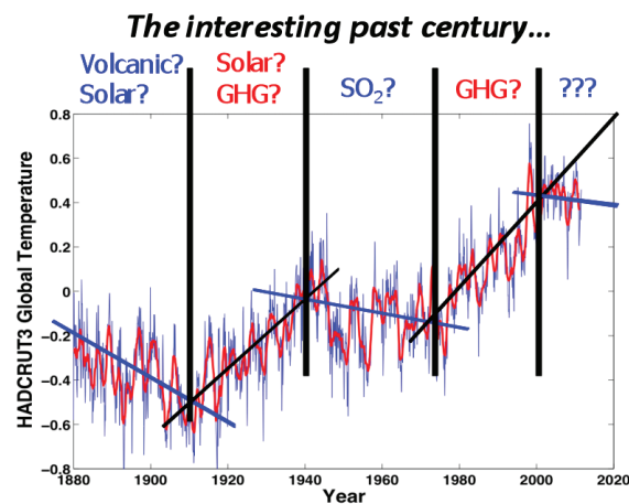
Figure 6: The past century has had some interesting trends in the global surface temperature record. Multi-component forcing can produce trend shifts, some up and some down, as different forcings appear to dominate. Currently, there is an unusually calm period in global surface warming change according to Kyle Swanson [UWM].
