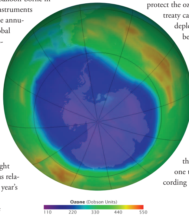
This image shows the extent, or geographic area, of the ozone hole at its widest on September 12, 2011, when it stretched 10.05 million mi 2 (26.03 million km 2 ). The lowest concentration of ozone in the southern stratosphere—that is, the deepest “hole”—occurred on October 9, 2011, when levels descended to 95 Dobson units. Image credit: NASA Ozone Watch
