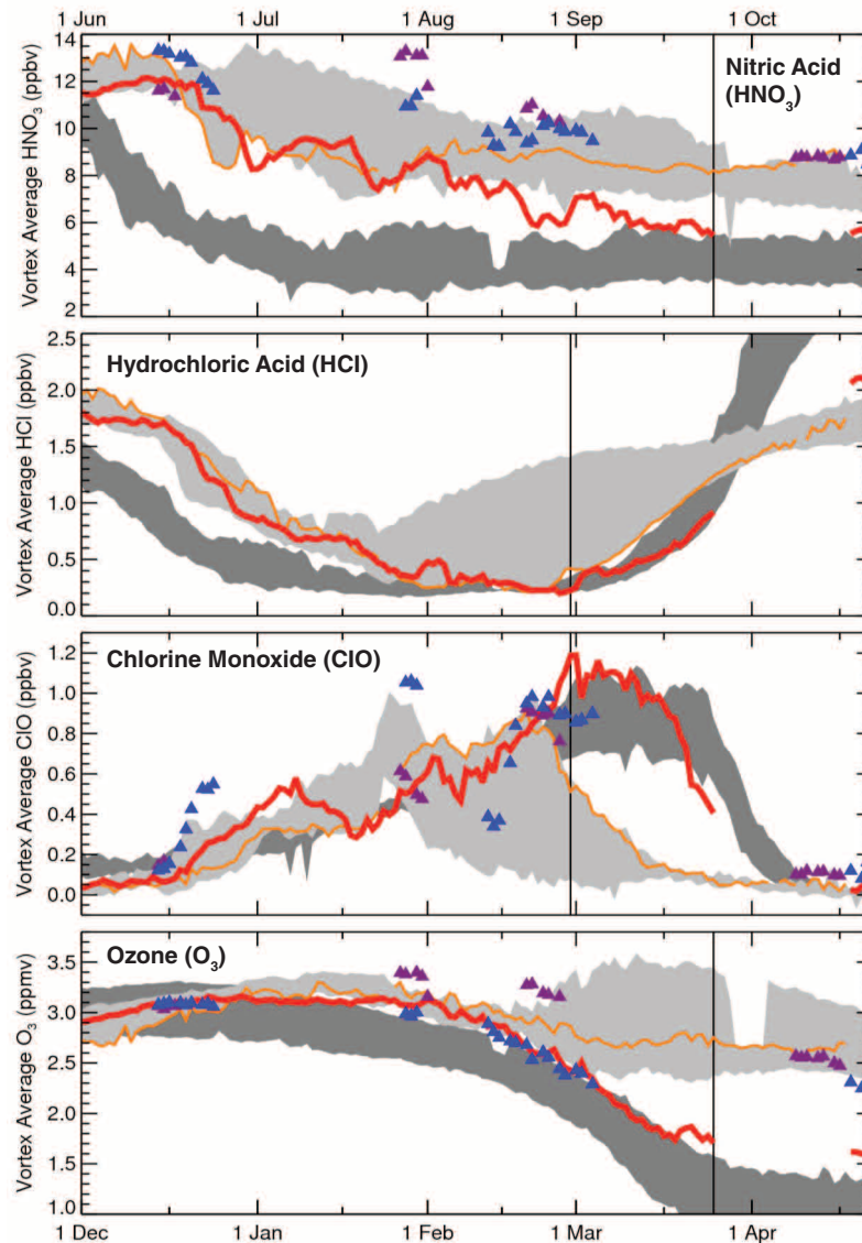
Figure 1: These MLS measurements show the unusual evolution of O_3 , ClO, HCl, and HNO_3 during Arctic spring of 2011.
