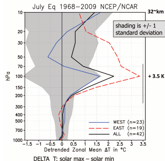
Figure 4: The solar-QBO relationship is shown as a function of altitude. The QBO East has a stronger solar signature according to Karin Labitzke [Freie Univ. Berlin]
