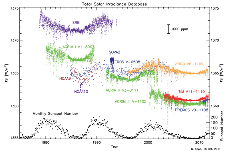
Figure 1: Recent calibration efforts by the Active Cavity Radiometer Irradiance Monitor (ACRIM), PREcision Monitoring Sensor (PREMOS), and Total Irradiance Monitor (TIM) teams have improved understanding of the offsets between Total Solar Irradiance (TSI) instruments. After corrections that are largely due to internal instrument scatter, the latest on-orbit TSI values agree well, Dick Willson (ACRIM3), Werner Schmutz (PREMOS), and Greg Kopp (TIM), all discussed these calibration efforts during Session I .
